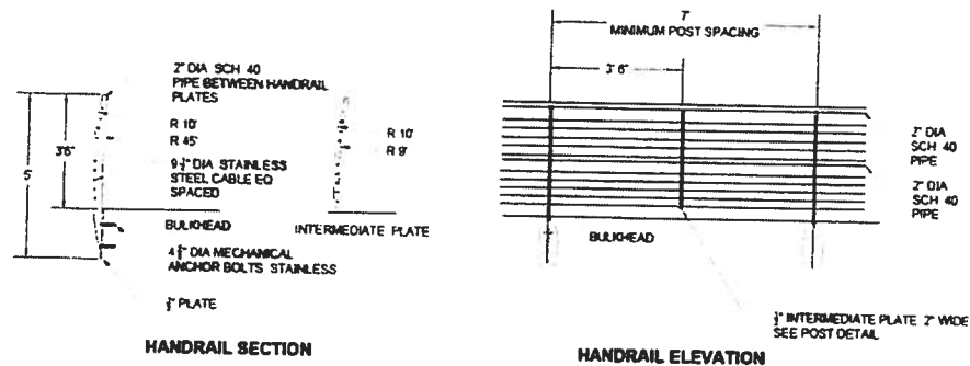
Example of acceptable Southbank Riverwalk railing mounted to a bulkhead.
